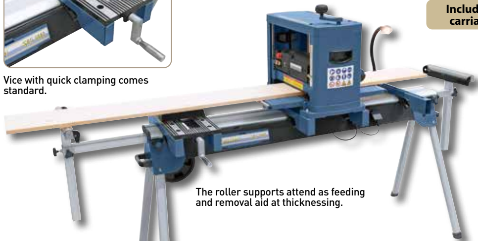
The moveable mounting rails can be adjusted quickly and easily to the machine width
