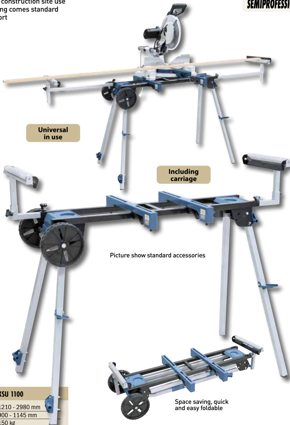
Roller supports stepless extractable and height adjustable on both sides
