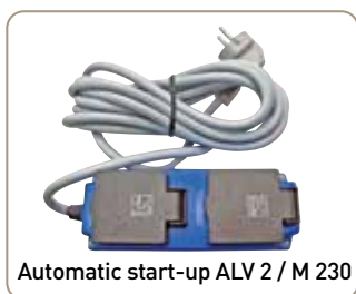
Automatic start-up ALV 2 / M 230 When switching the wood working machine on / off, the radial collector automatically turns on / off with delay. (optional extra)
