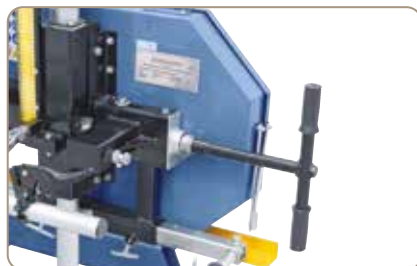
User-friendly tensioning of bandsaw blade, easy to access.
